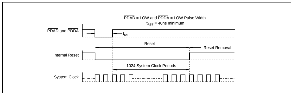
FIGURE 6. External Forced Reset Timing.
